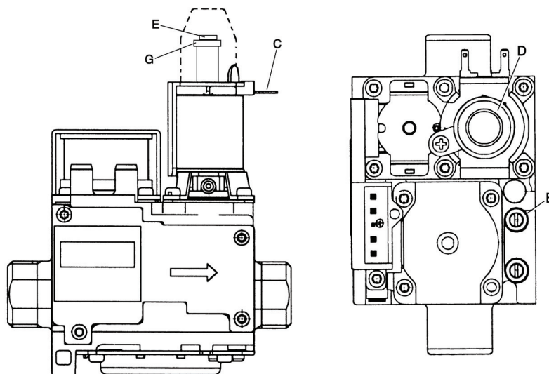
fig. 18 - Valvola gas
