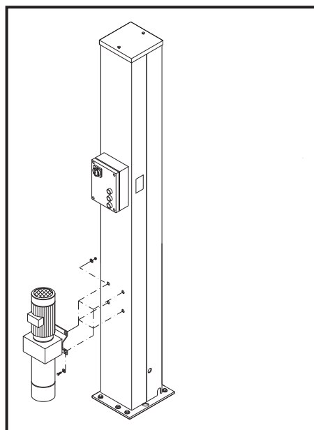
Fig.39 Hydraulic oil unit assembly
