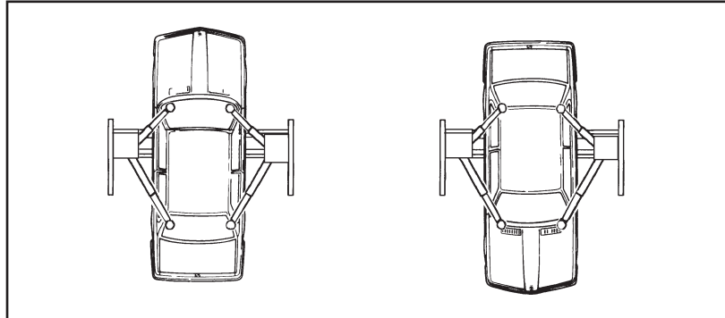
Fig.16 Correctly loaded vehicle
