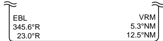
Figure 2-6 Display bottom, showing location of EBL and VRM readouts
