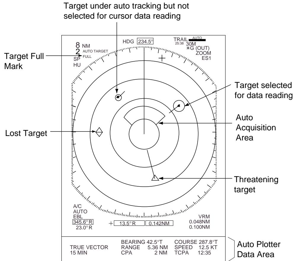
Figure 6-2 ARPA display
