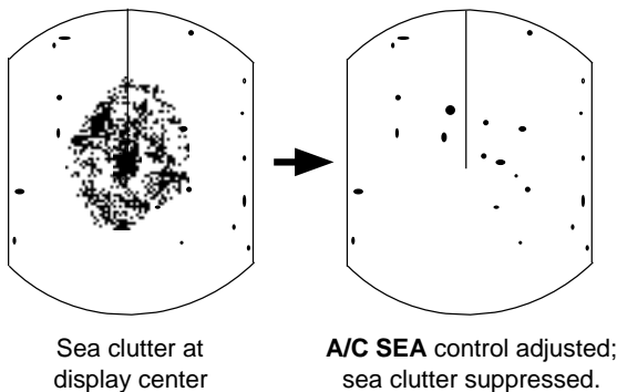
Figure 2-3 How to adjust the A/C SEA control
