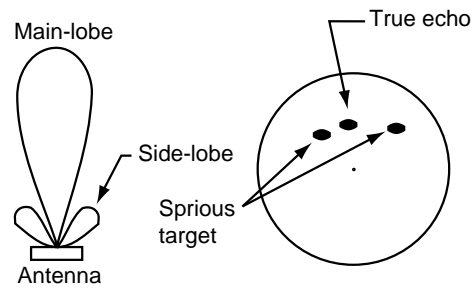
Figure 4-2 Side-lobe echoes
