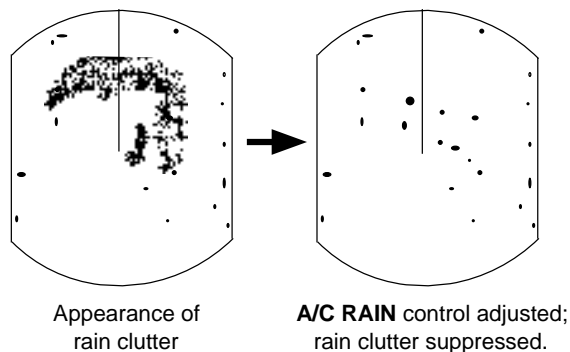
Figure 2-4 Effect of A/C RAIN
