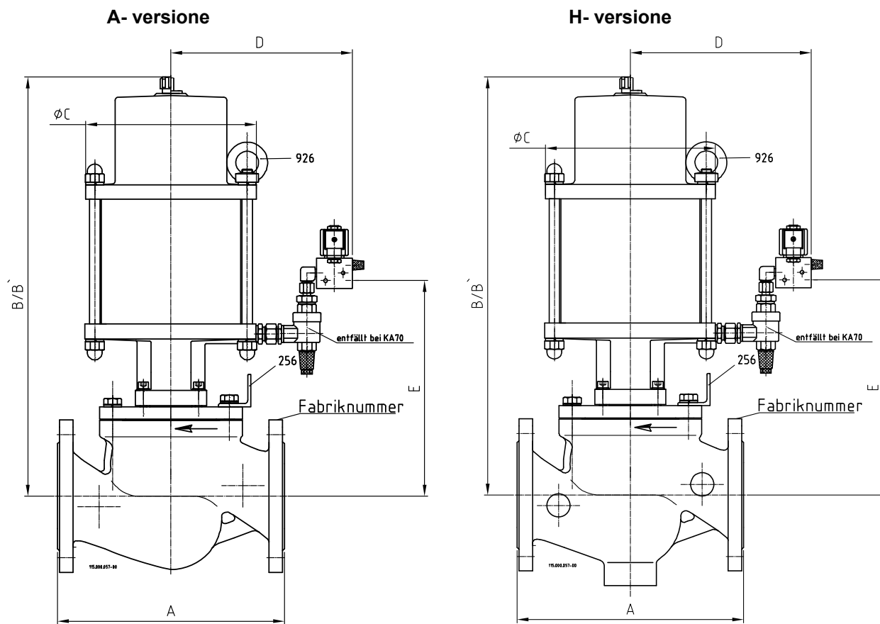
...-4-EPVA...N(H).. in Fig. 2
