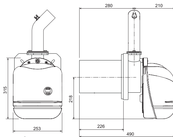
fig. 14 - Dimensional SUN P7
