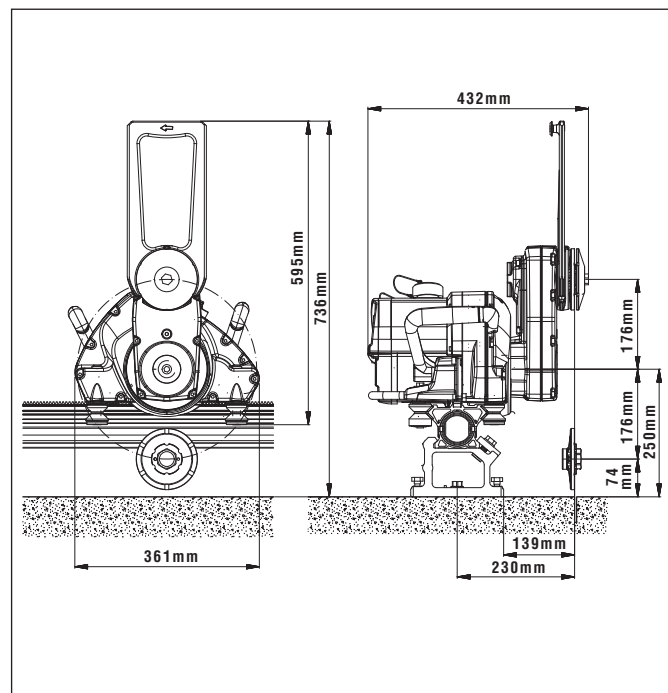
Dimensioni e misure DS TS20-E (in mm)
