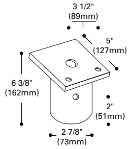
TKS=Slipfitter Adapter 3 (Fits 2 3/8" O.D. Tennon)
