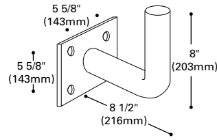
RAB=Right Angle Pipe Bracket 3 (2 5/8" O.D.)
