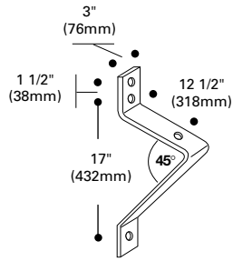
SAB=Steel Angle Bracket 3
