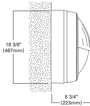
SHALLOW CASTING (Units with CSTG, F1 Option, EM & SC Option and SCB18 Accessory)
