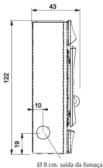
LATERAL
