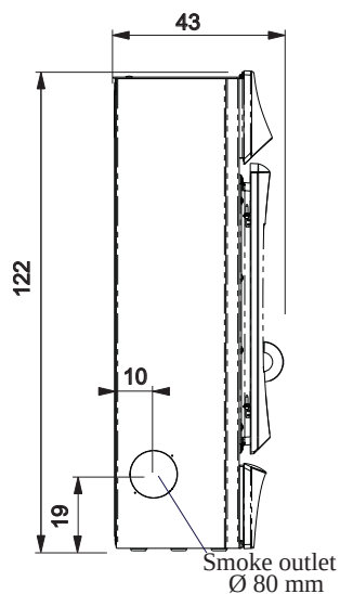
SIDE
