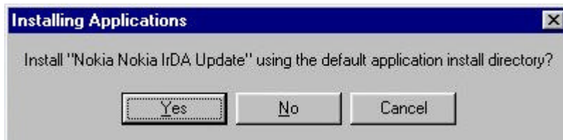
Figure 4: Installing applications.
