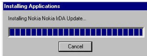
Figure 5: Installing files.
