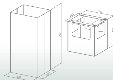
KIT SUP. ISOLA H700 X
