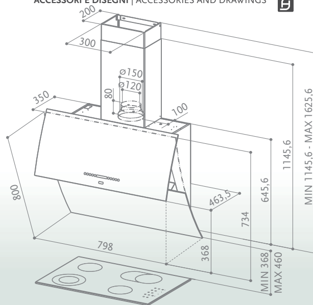
MIRROR - MIRROR ART
