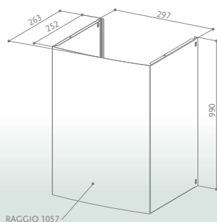
KIT ARCO PLUS H990 X
