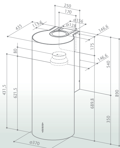
CYLINDRA - CYLINDRA GLOSS
