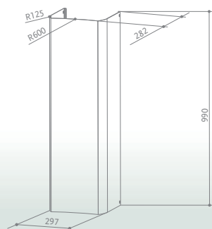
KIT AXIA PLUS H990 X
