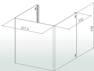
KIT H990 X
