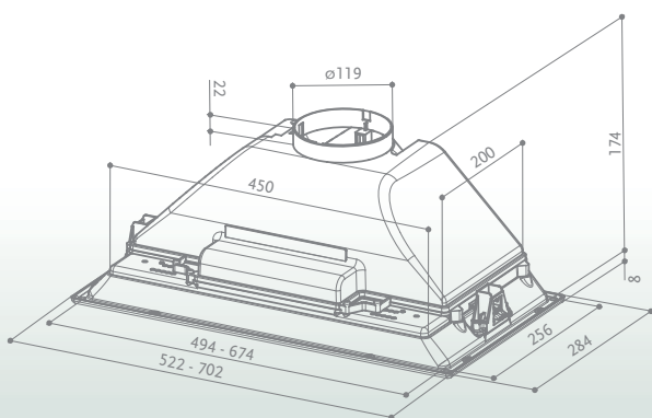
INCA SMART - INCA SMART C / HC / HCS
