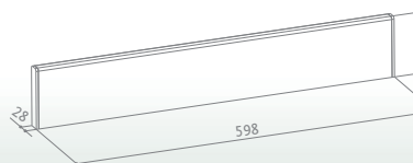
KIT FRONTALE H15 60 CM BK
