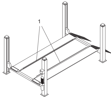
Fig.24 Side movements and platform kerbs
