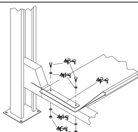
Fig.63 Securing the vehicle ramps and wheel stops
