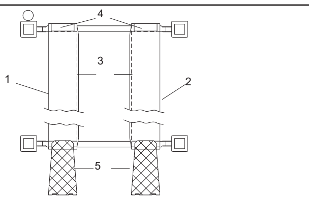
Fig.11 Platforms and cross-pieces
