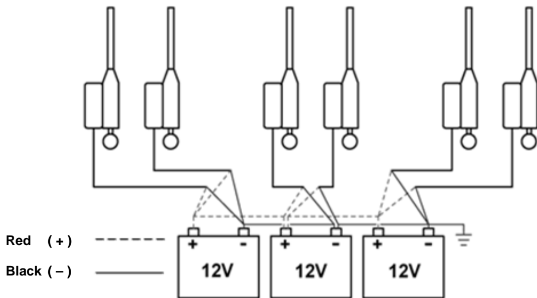
Connect Multiple Batteries in Parallel
