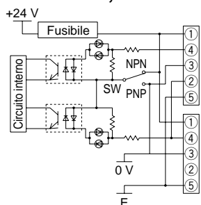
Diagramma circuito: EX250-IE1
