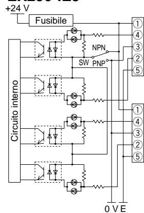
Diagramma circuito: EX250-IE2
