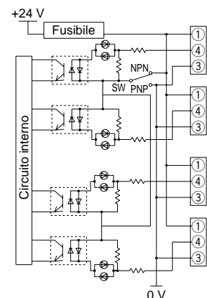
Diagramma circuito: EX250-IE3
