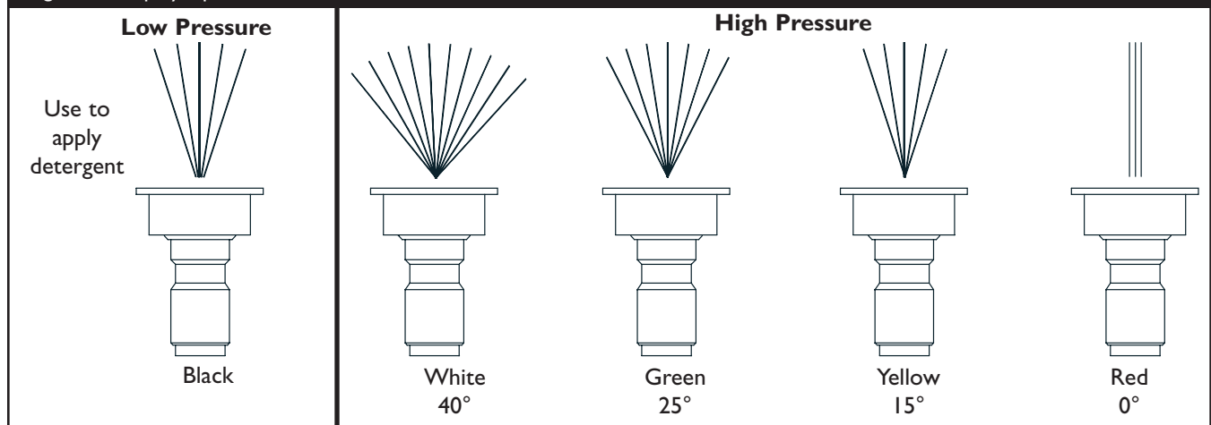
Figure 8 — Spray Tips
