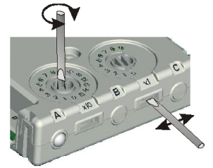
FIGURE 3: M710-CZR CONVENTIONAL ZONE INTERFACE MODULE
