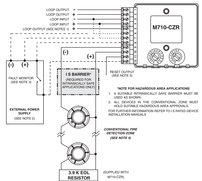
FIGURE 3: M710-CZR CONVENTIONAL ZONE INTERFACE MODULE
