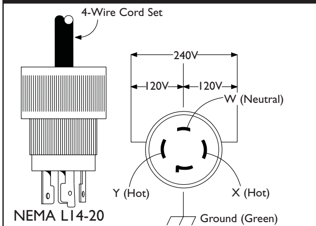
Figure 8 — 120/240 Volt AC, 20 Amp Receptacle
