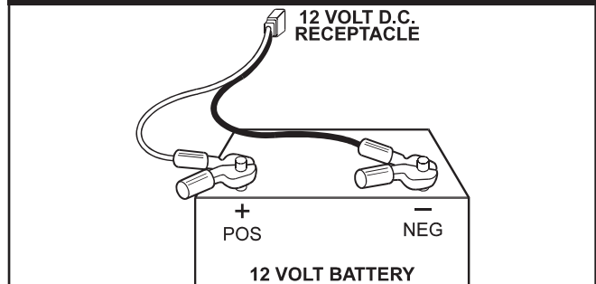
Figure 6 — Battery Connections
