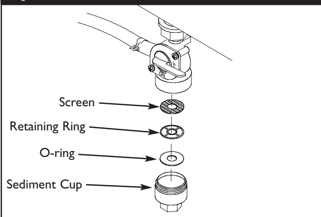
Figure 14 — Fuel Valve Maintenance
