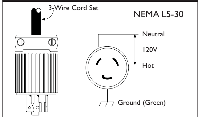
Figure 9 — 120 Volt AC, 30 Amp, Locking Receptacle
