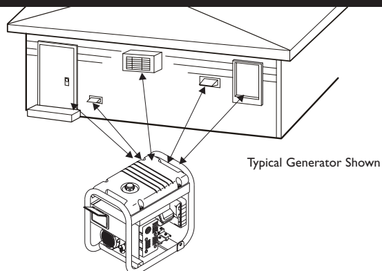
Figure 3 — Generator Clearance
