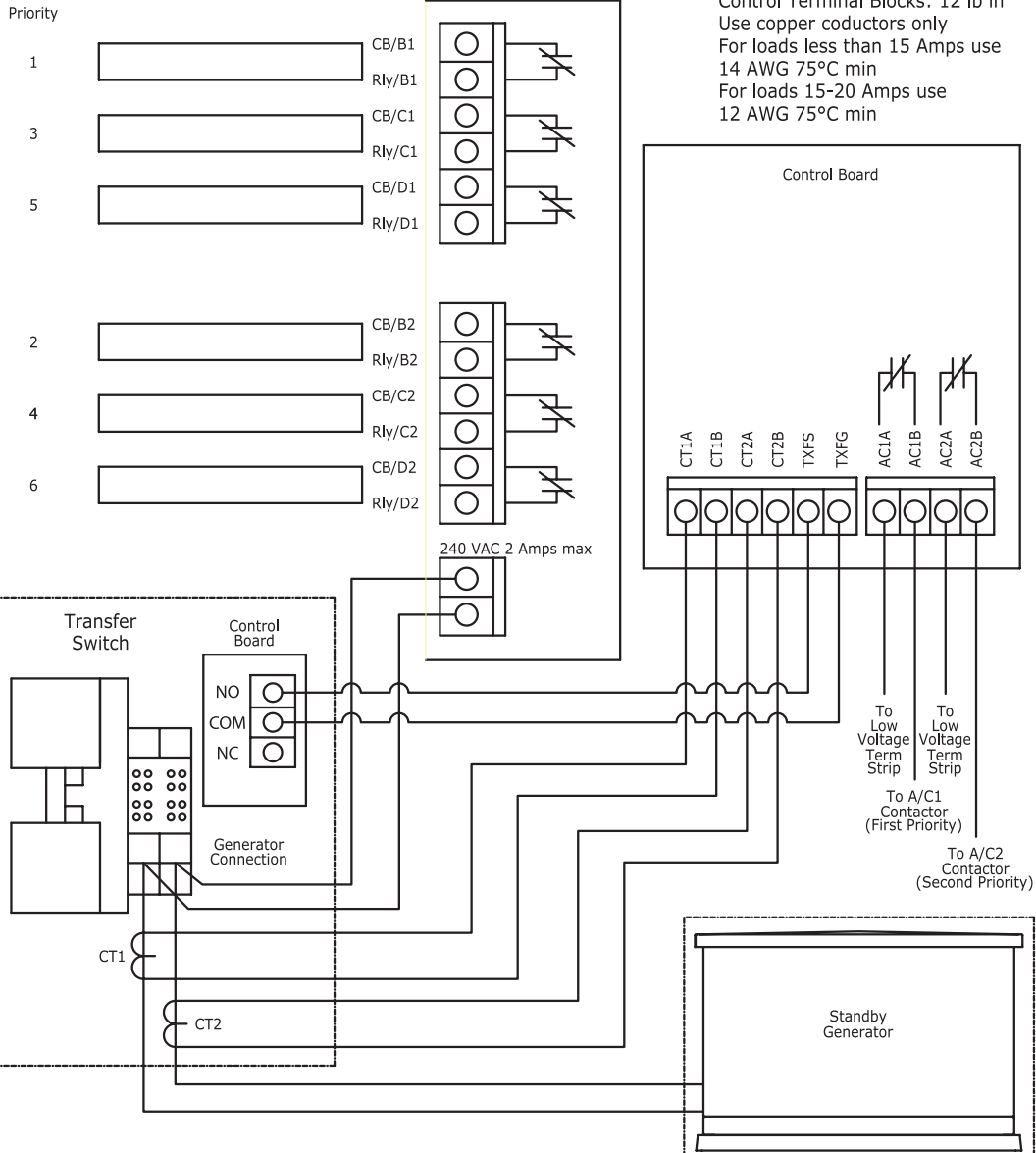
Contactor Example: Typical control of 240VAC load
