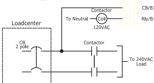
Contactor Example: Typical control of 240VAC load
