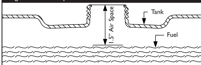
Figure 2 - Fuel Expansion
