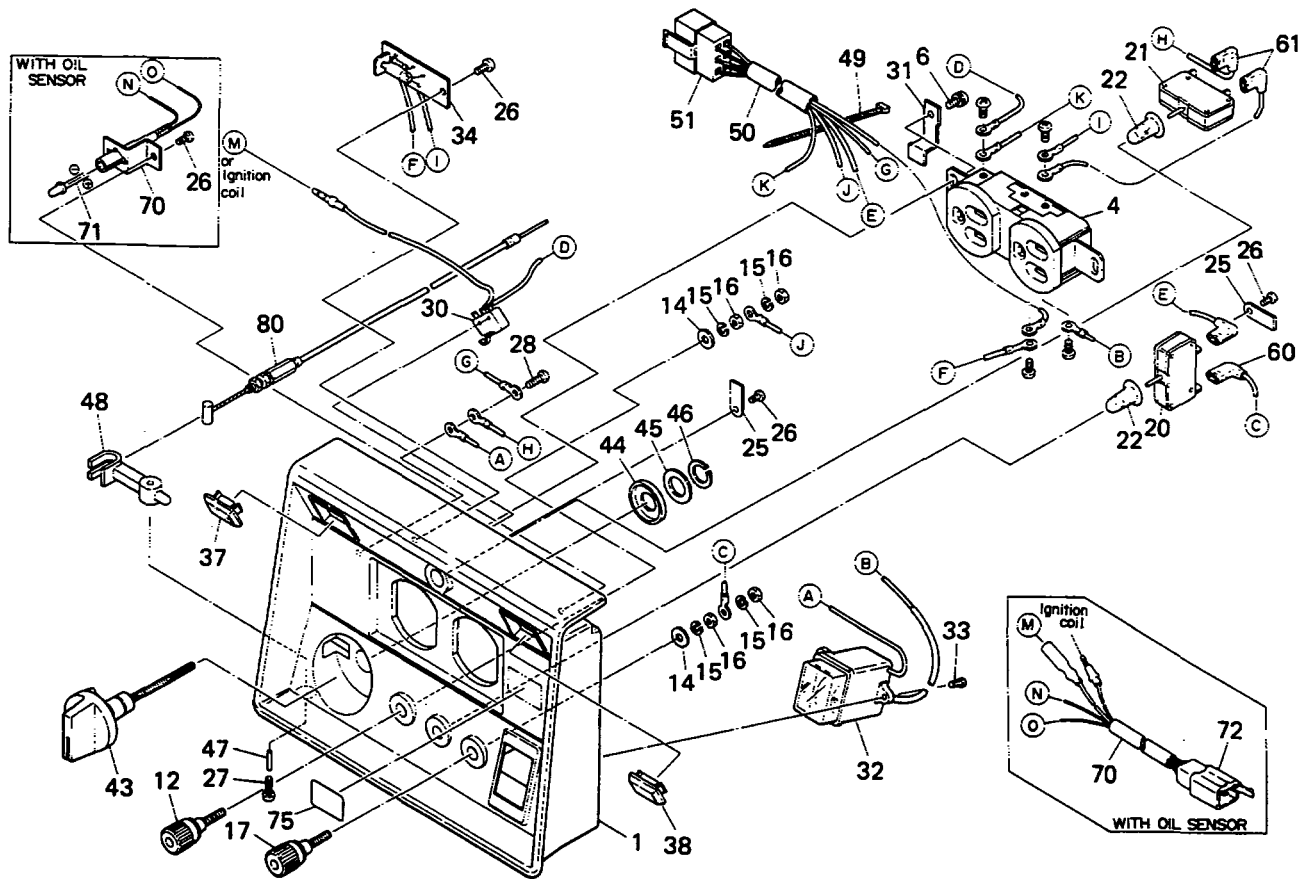
Fig. 2-1 CONTROL PANEL
