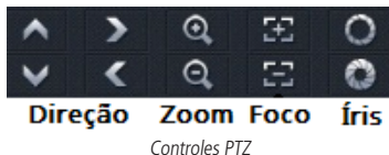
Controles PTZ
