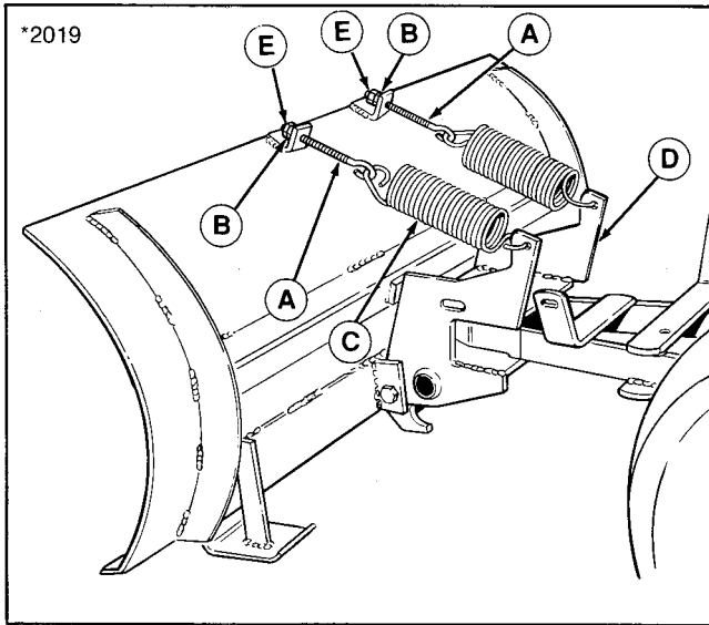
Figure 2. Tension Springs
