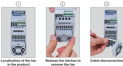
Figure 6.1: Removal of the heatsink fans
