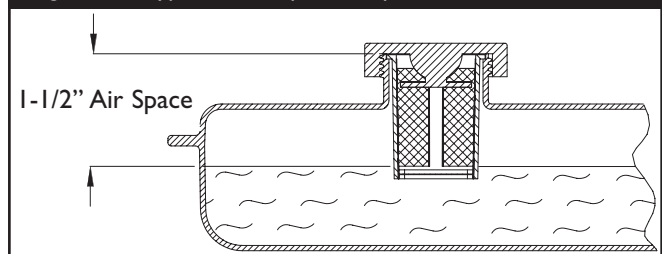
Figure 1 — Typical Fuel Expansion Space
