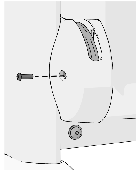
Figure 6: Kick plate pulley cover removal
