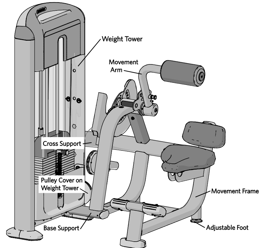
Figure 1: Back Extension components
