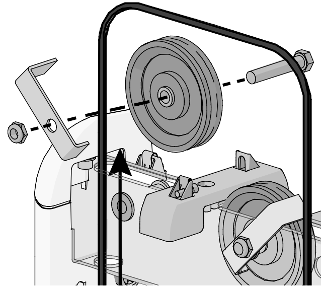
Figure 10: Removal of pulley and cable retainer
