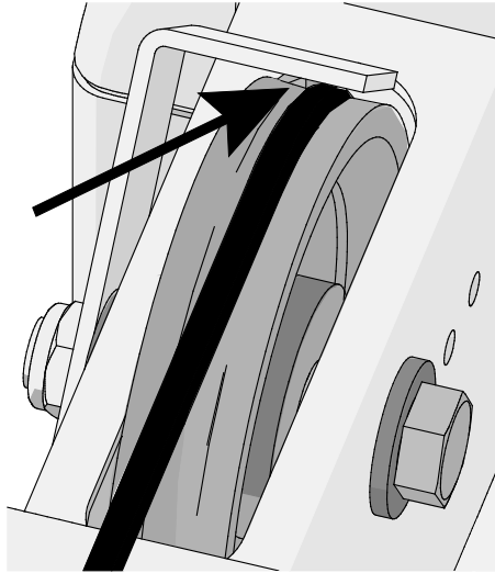
Figure 11: Proper position of cable under cable retainer
