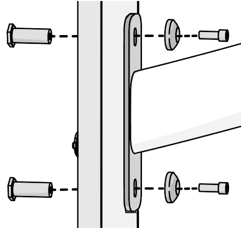
Figure 3: Cross support attachment to weight tower
