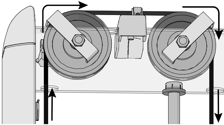
Figure 9: Position of cable over pulleys
