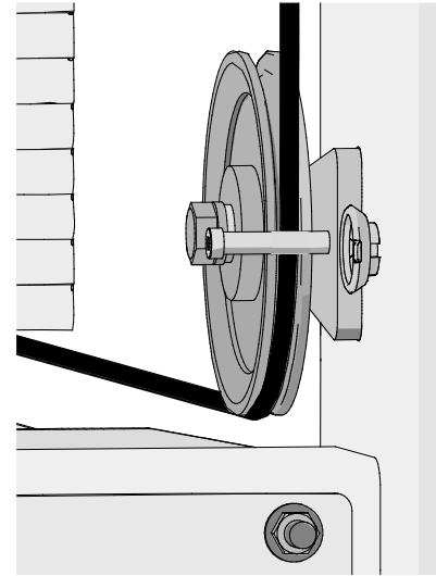
Figure 8: Cable and shoulder bolt position
