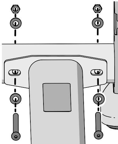
Figure 2: Base support attachment to weight tower
