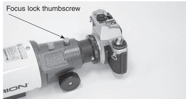
Figure 3. The ShortTube 80-A with 35mm SLR camera attached.
