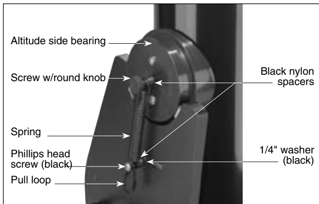
Figure 13. Close-up view of the CorrecTension system.
