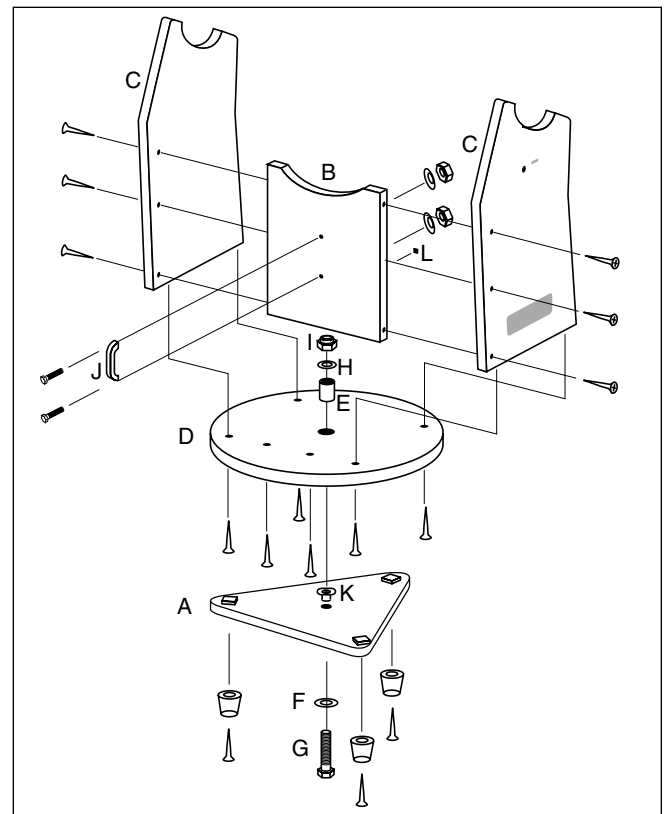
Figure 9. Exploded view of the Dobsonian base.
