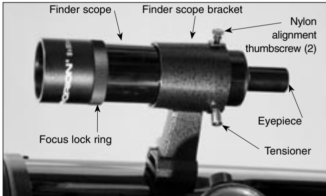
Figure 15a. The 9x50 finder scope and bracket.
