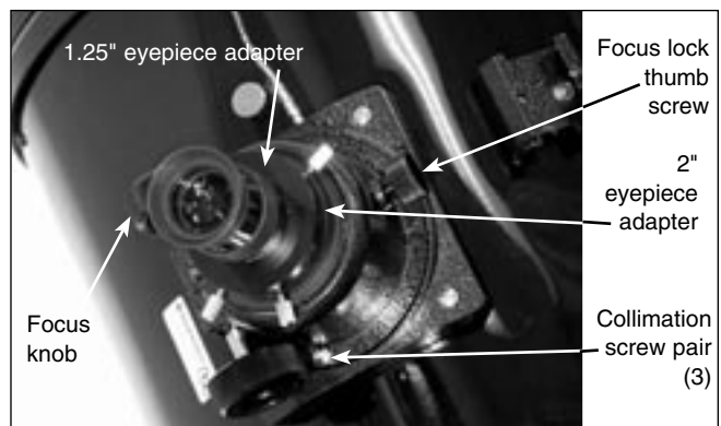
Figure 16. The large format focuser with eyepiece adapters attached. The focuser will accept eyepieces with barrel diameters of both 1.25" and 2".
