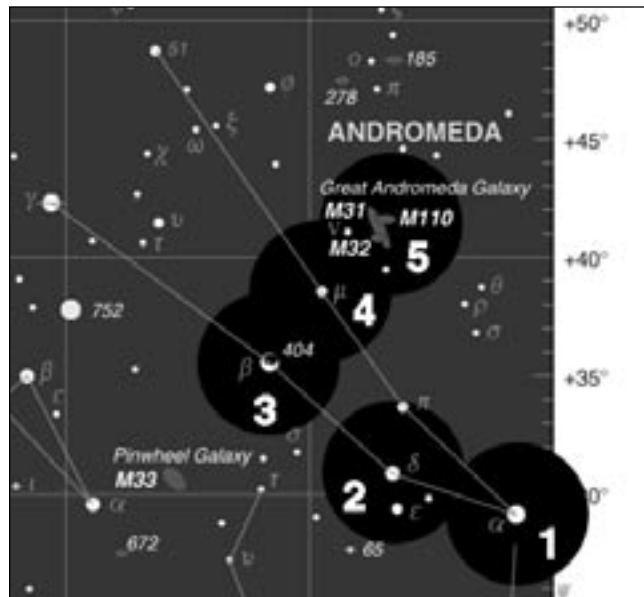
Figure 25. Starhopping is a good way to locate hard-to-find objects. Refer to a star chart to map a route to the object that uses bright stars as guideposts. Center the first star you’ve chosen in the finder scope and telescope eyepiece (1). Now move the scope carefully in the direction of the next bright star (2), until it is centered. Repeat (3 and 4). The last hop (5) should place the desired object in the eyepiece.
