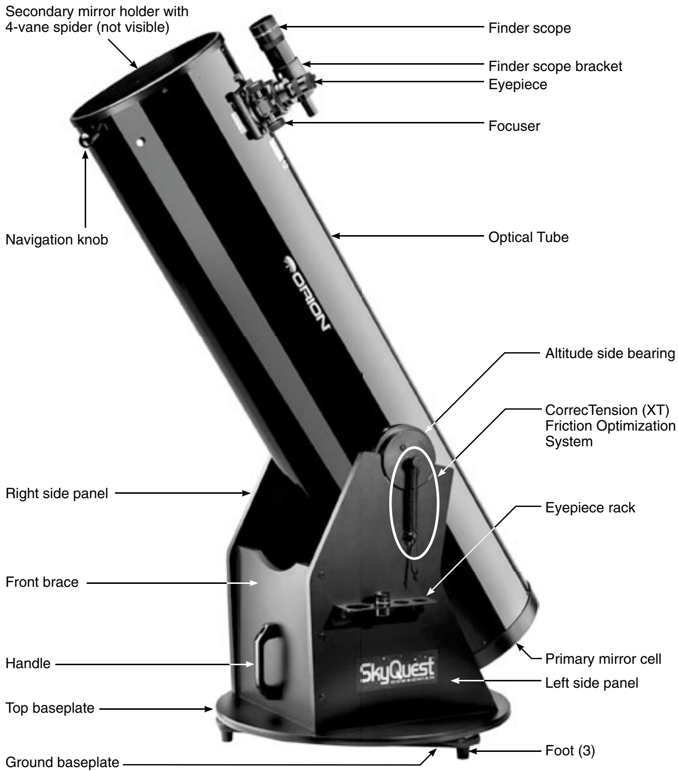
Figure 1. The SkyQuest XT12 Classic Dobsonian.
