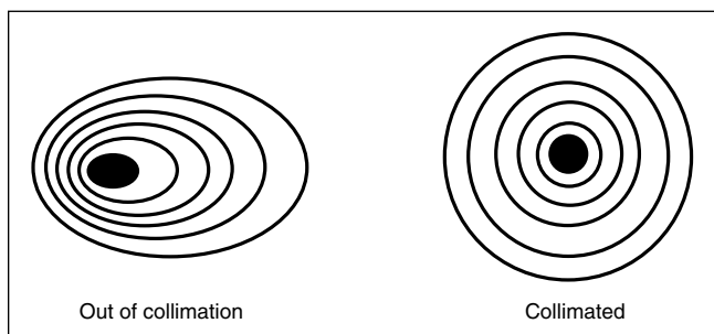
Figure 24. A star test will determine if a telescope’s optics are properly collimated. An unfocused view of a bright star through the eyepiece should appear as illustrated on right if optics are perfectly collimated. If circle is unsymmetrical, as in illustration on left, scope needs collimation.
