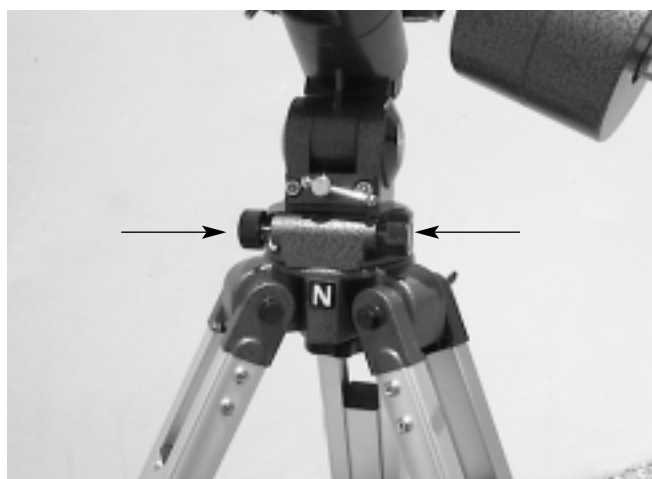
Figure 9. For polar alignment, position the telescope so that the “N” label at the base of the mount faces north. The two azimuth adjustment knobs above it (arrows) are used to make fine adjustments to the mount’s azimuth position.
