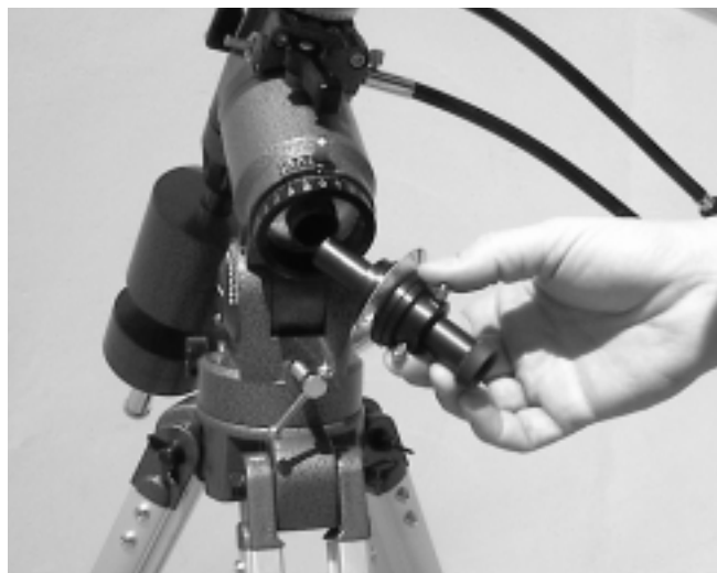
Figure 4. You may find it easier to install the polar axis finder scope by unthreading the rear part of the R.A. housing, inserting the finder in it, then rethreading the assembly back on the mount.
