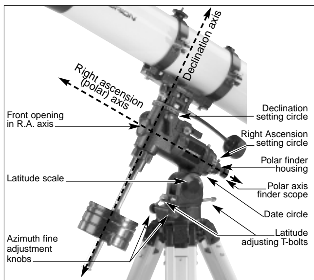
Figure 7. The equatorial mount of the AstroView 120 EQ.
