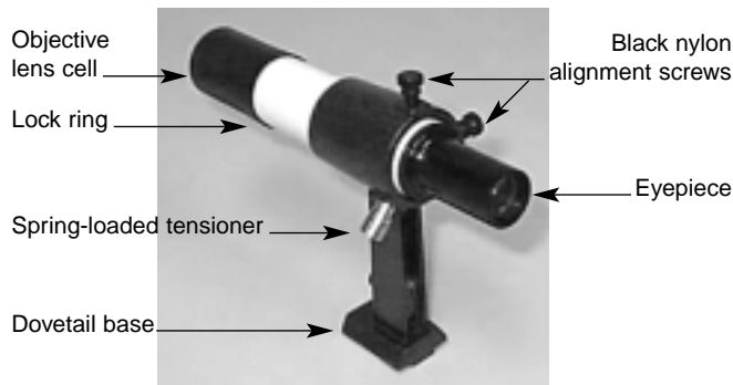
Figure 6. The 6x30 achromatic finder scope fits inside an aluminum dovetail bracket.
