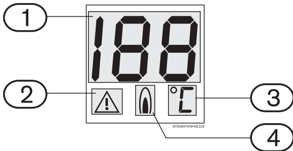
Fig. 6 Visor digital
