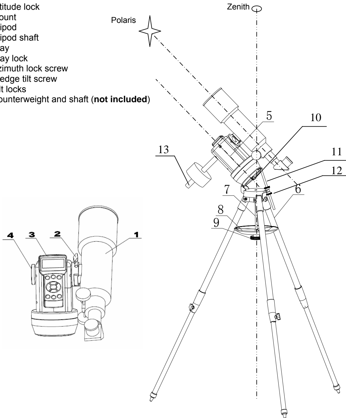
Figure 1. Assembly Terms
