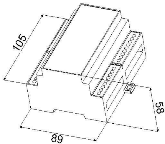
Figura II.4 – Dimensional do Multi-Point
