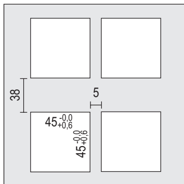
Recorte do Painel C704 (mm)
