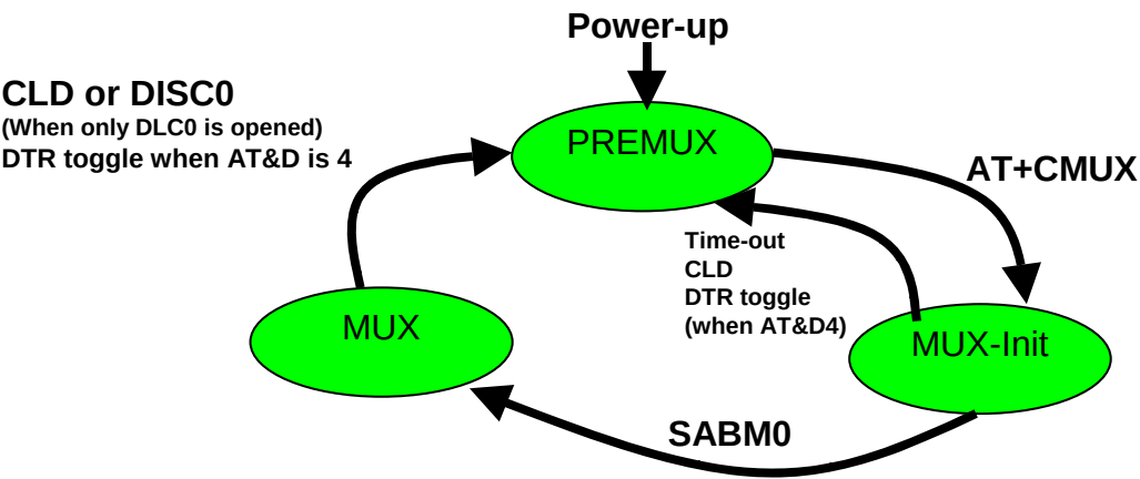
Figure 3-20: MUX States
