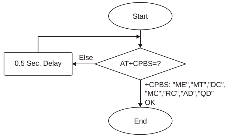
Figure 4-9: Terminal Synchronization
