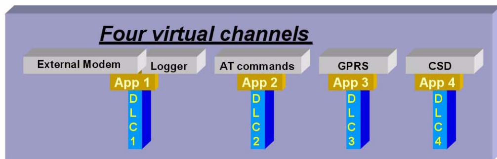
Figure 3-22: Four-Channel Configuration
