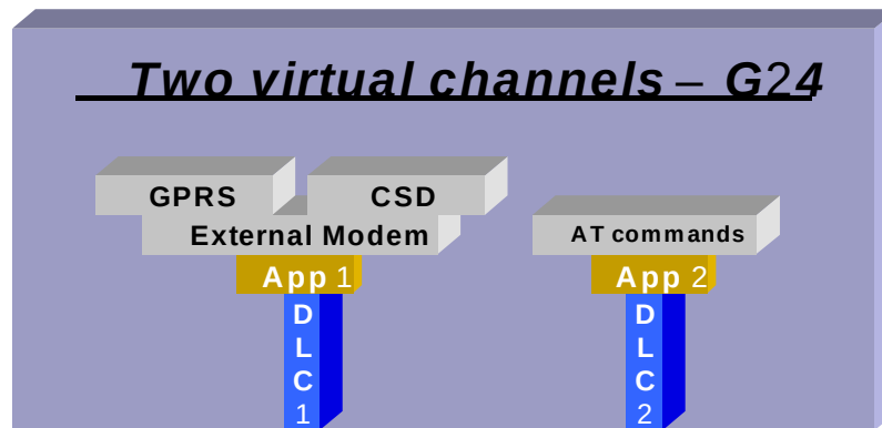
Figure 3-21: Two-channel Configuration
