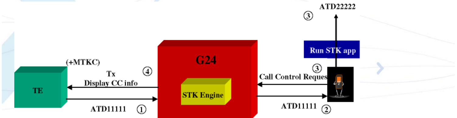
Figure 4-20: Call Control
