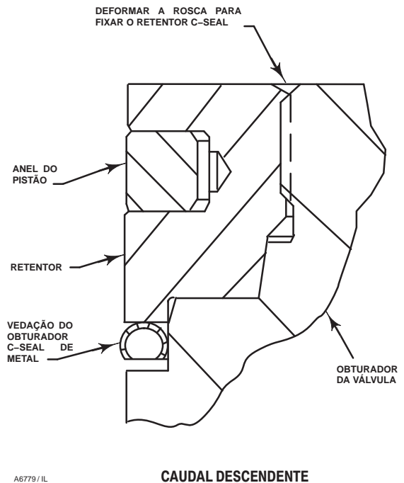
Figura 12. Fixar as Roscas do Retentor C-seal
