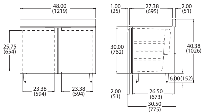
UF-48-SBS FRONT VIEW
