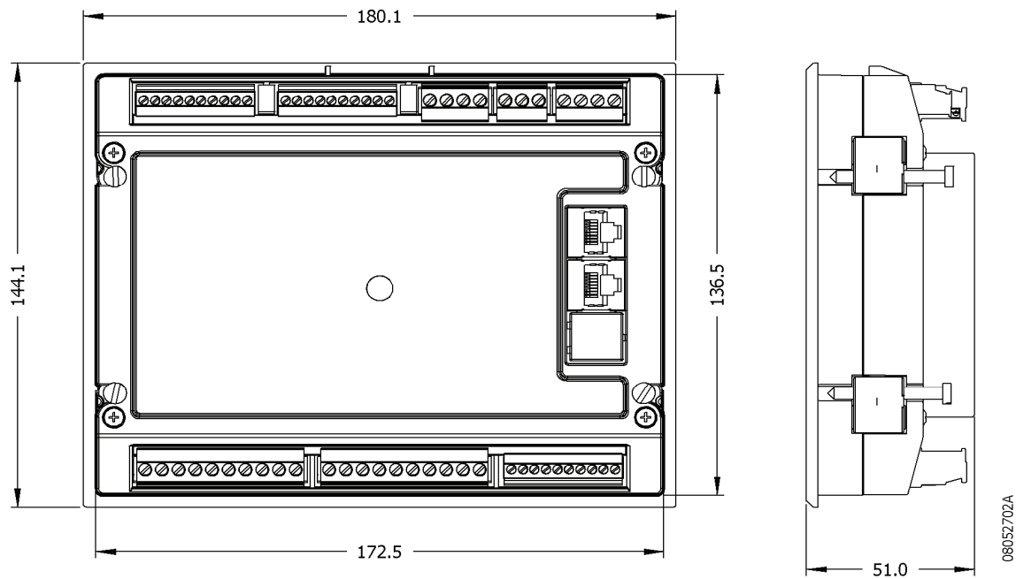
Figura 2-1. Dimensional CPS4310/R42 e T42
