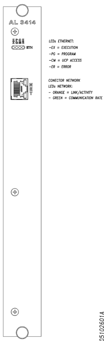
Figura 2-1. AL-3414 - Painel frontal
