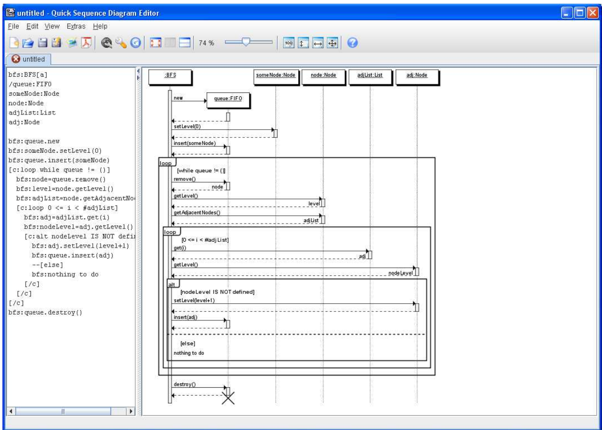
Figura 40 - Janela do Quick Sequence Diagram Editor
