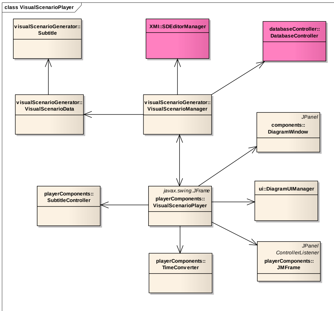
Figura 45 - Diagrama de classes do pacote playerComponents
