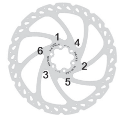
Disc Screw Torquing Sequence
