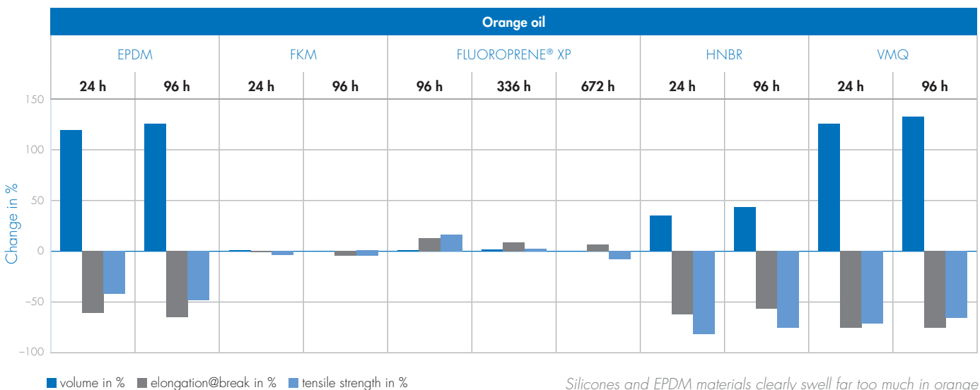
IMMERSION RESULTS OF EPDM, FKM, FLUOROPRENE® XP, HNBR AND VMQ IN ORANGE OIL
