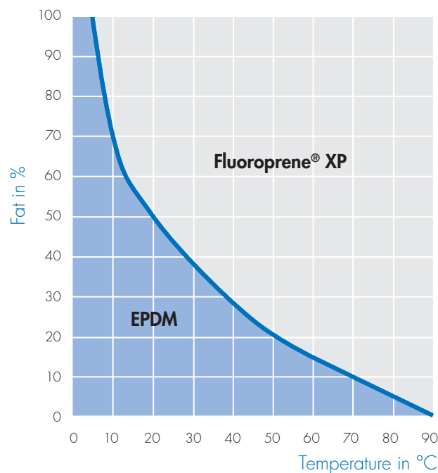
FAT CHART FOR EPDM
