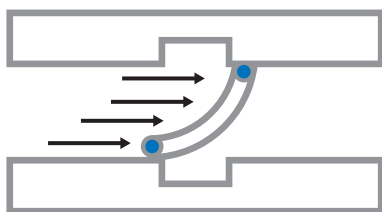
Inside sealing – grooves in housing
