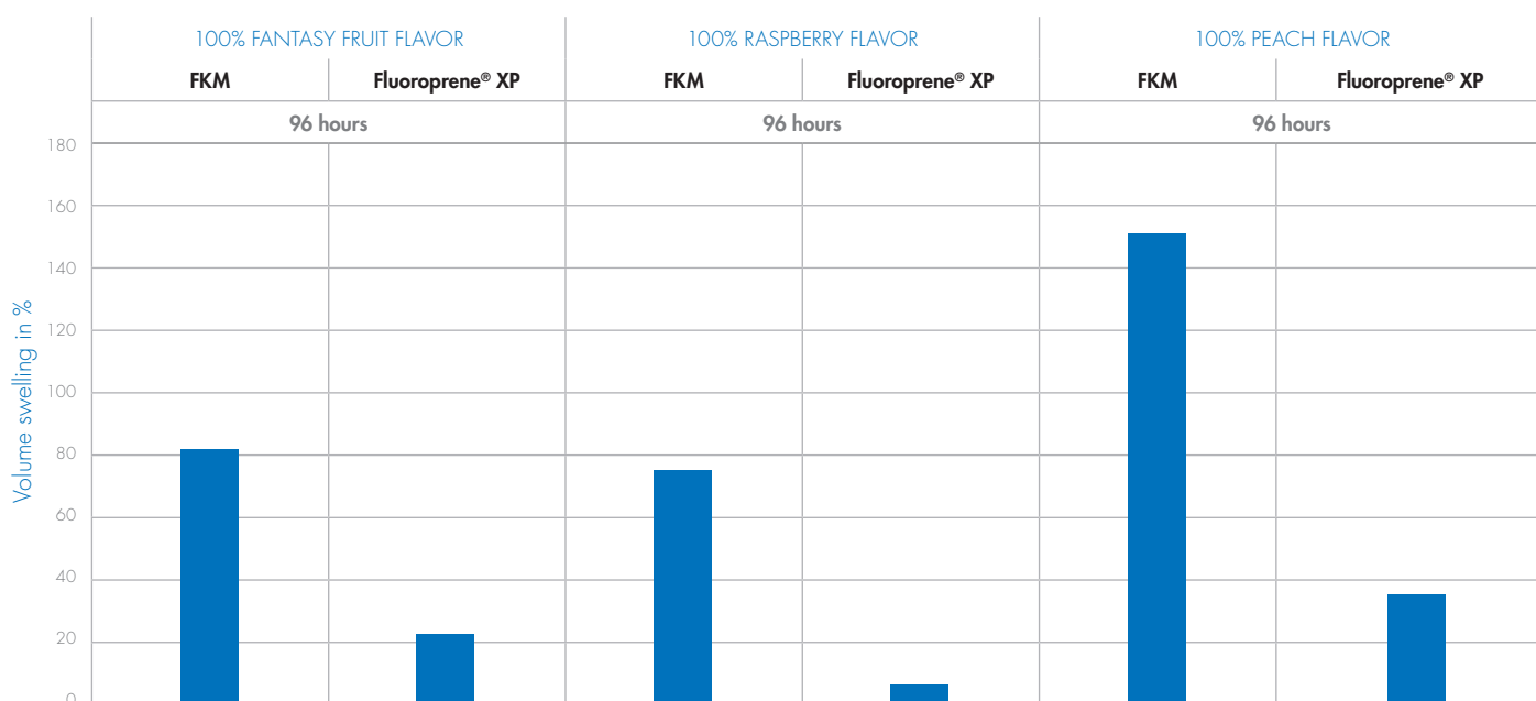
VOLUME CHANGE OF FKM AND FLUOROPRENE® XP IN DIFFERENT FLAVOR CONCENTRATES
