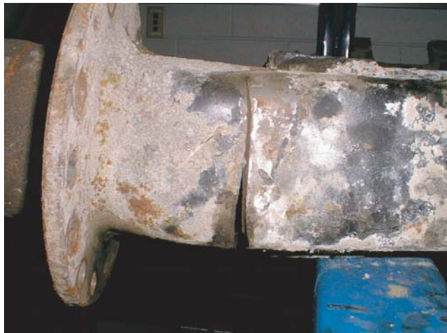
Housing Arm Fatigue
