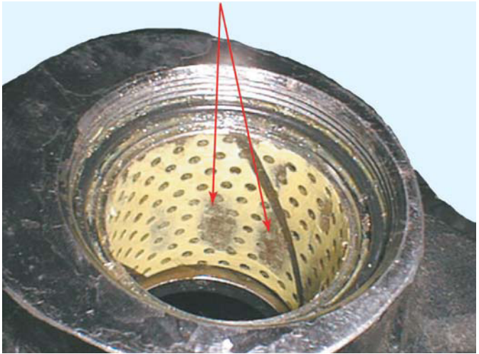
Improper Reaming
