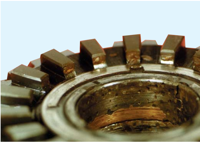
Helical Side Gear Wear - Water Contamination
