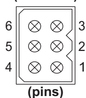
Control Side (end view)
