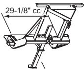
22240 RD/HD Headgear Kit
