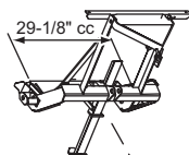
22135 Headgear Kit
