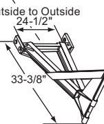
21484-1 Push Assembly (Part of 8440)
