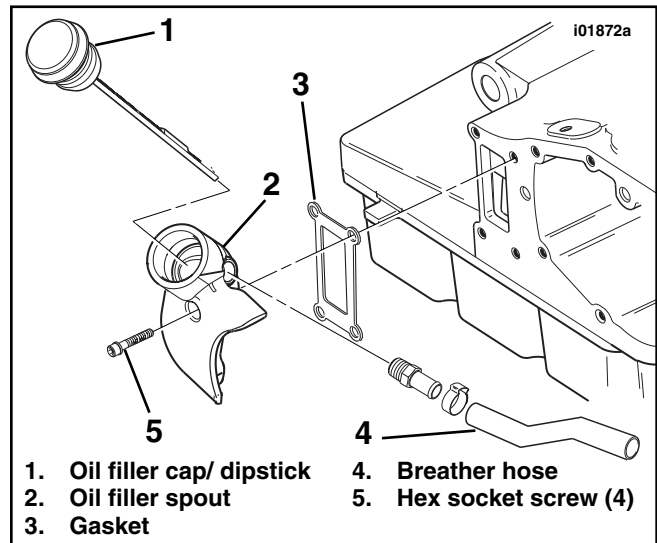
Figure 1. Remove Oil Filler Spout (FLT Only)
