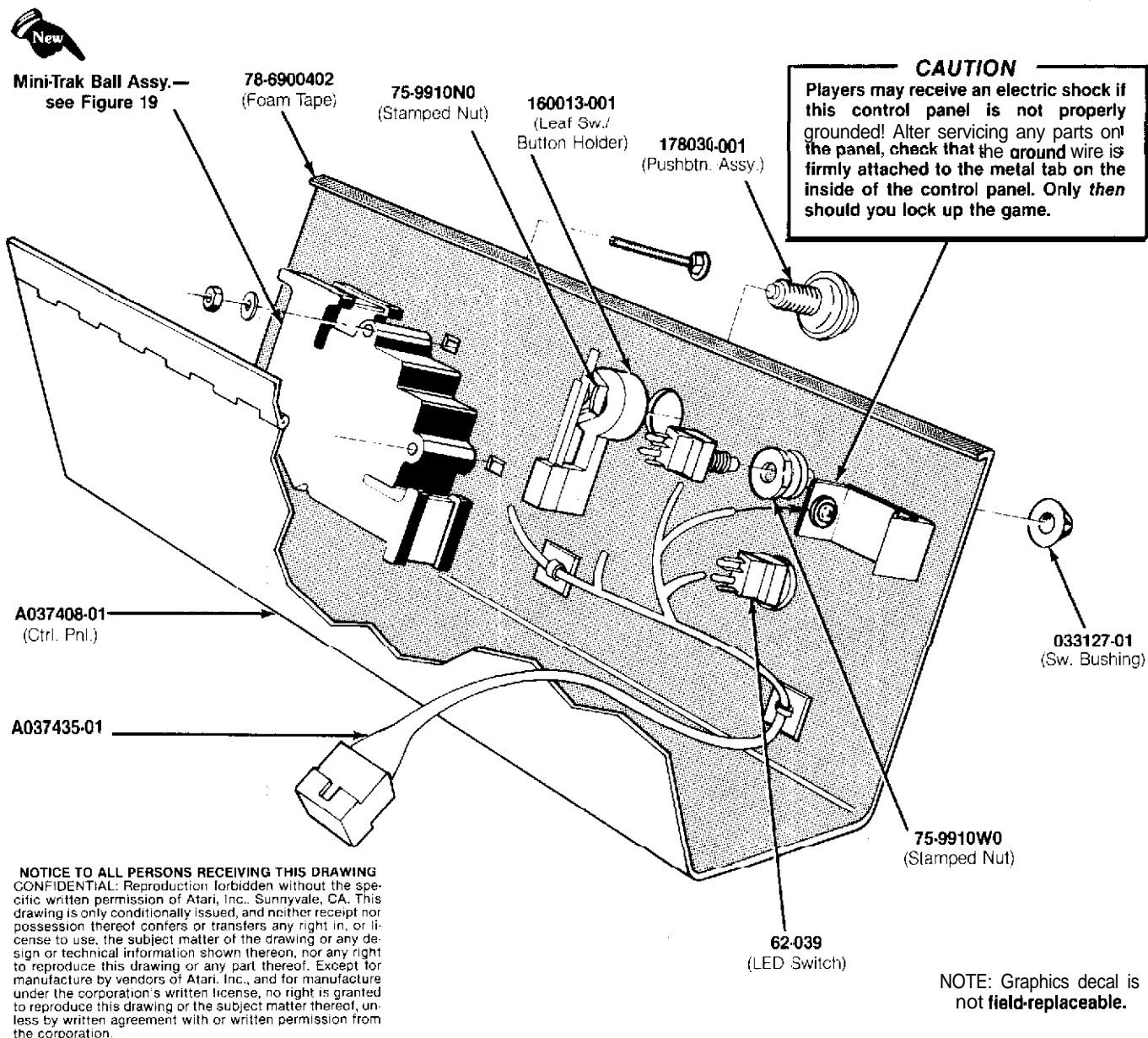
Figure 18 Control Panel Assembly A037409-01 A
