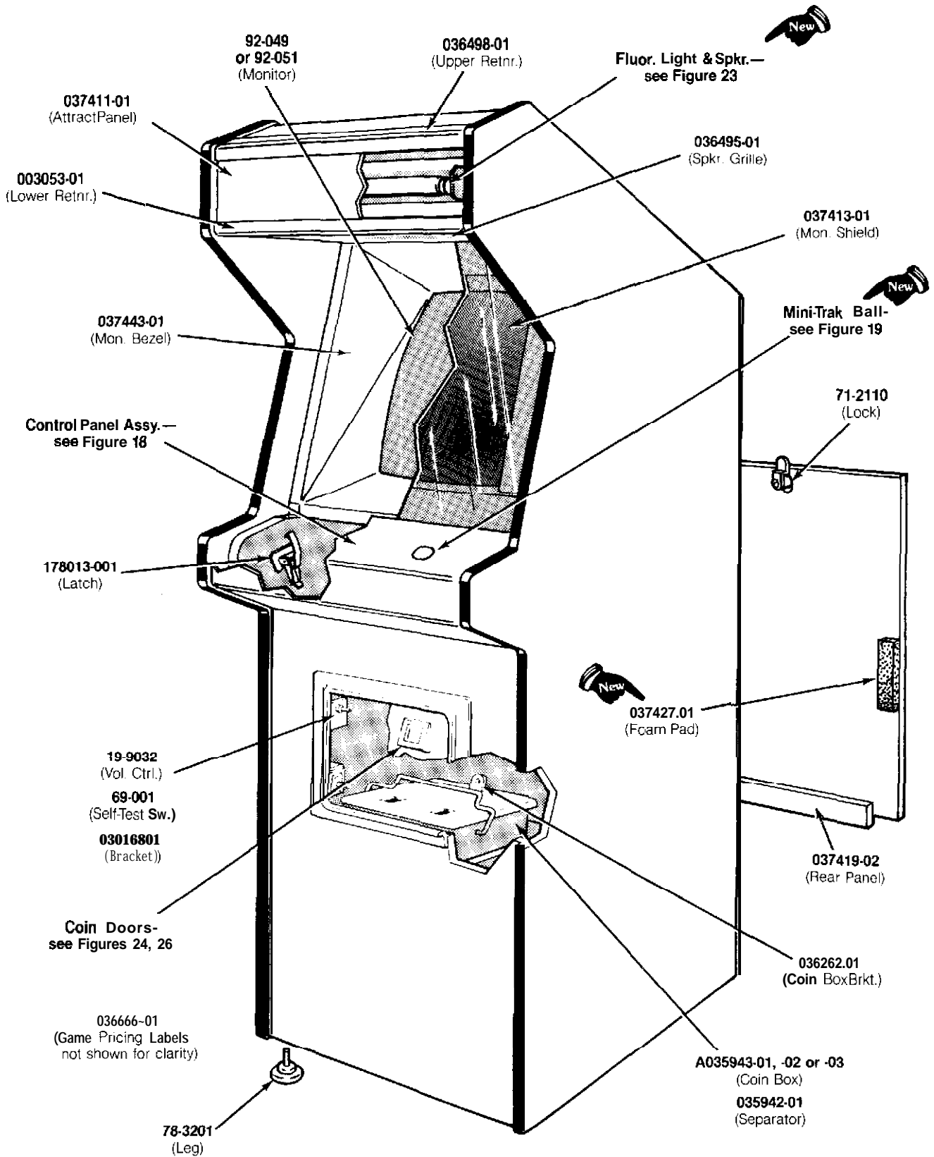
Figure 17 Cabinet-Mounted Assemblies A037397-xx A
