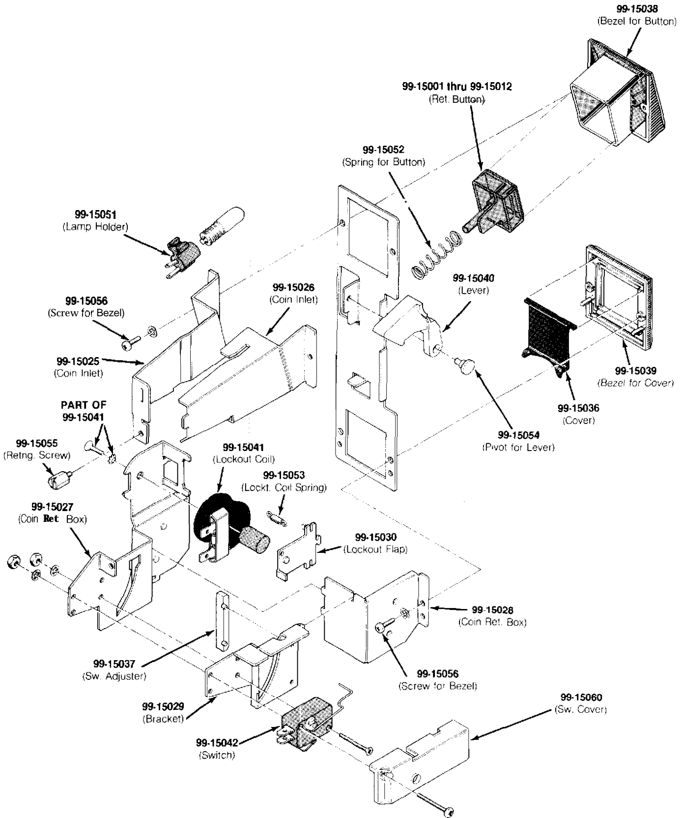
Figure 25 British-Made Coin Door 171001-xxx A
