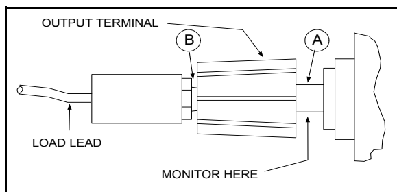
Figure A-2. Front Panel Terminal Connections
