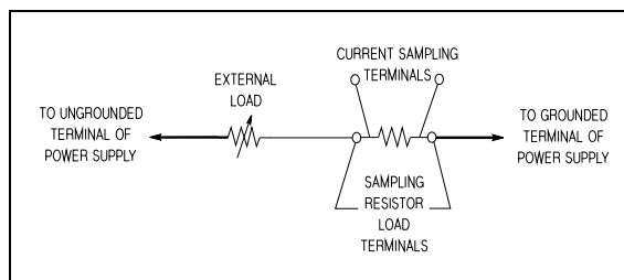
Figure A-3. Current Sampling Resistor Connections
