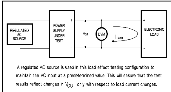
Figure A-5. Basic Test Setup
