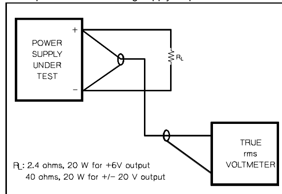
Figure A-6. Ripple and Noise rms Measurement Test Setup
