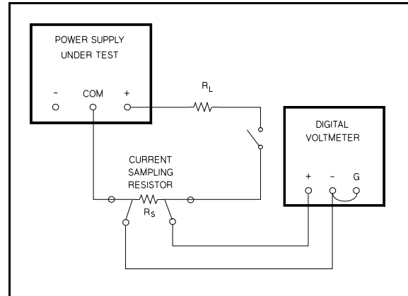
Figure A-4. Output Current, Test Set UP
