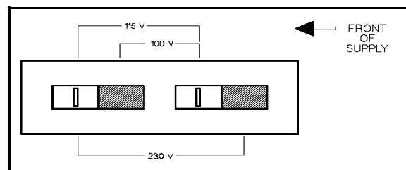
Figure A-1. Line Voltage Selector (set for 115 VAC)
