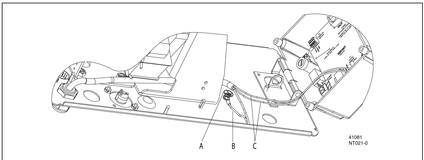
Figure 3: Installing Ground Wire on Transformer, 3150/3900 Valves
