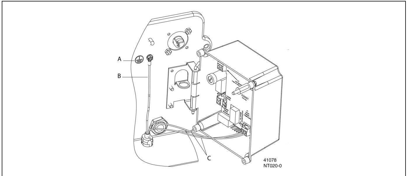
Figure 2: Installing Ground Wire on Transformer, 2750/2850/2900 Valves
