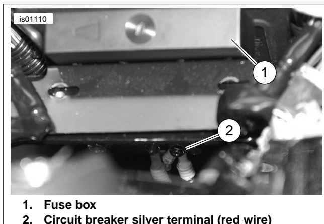
Figure 18. Circuit Breaker (2003 or Earlier Softails)
