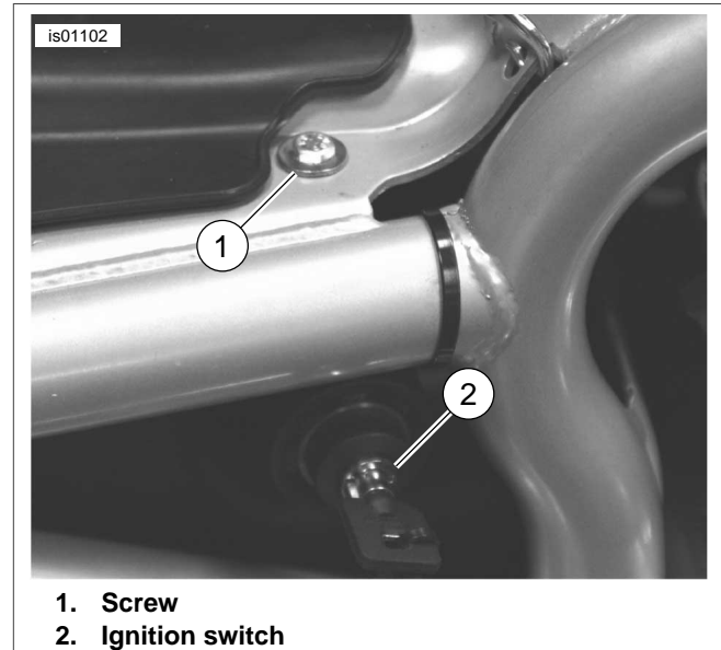
Figure 6. Ground Connection (2006 and Earlier V-Rod Models)
