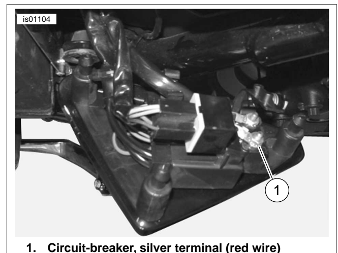
Figure 19. Circuit Breaker (2003 or Earlier Sportsters)
