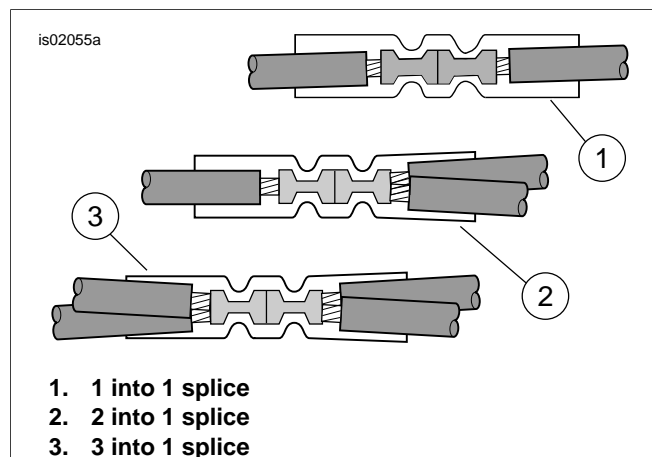
Figure 7. Splice Configurations
