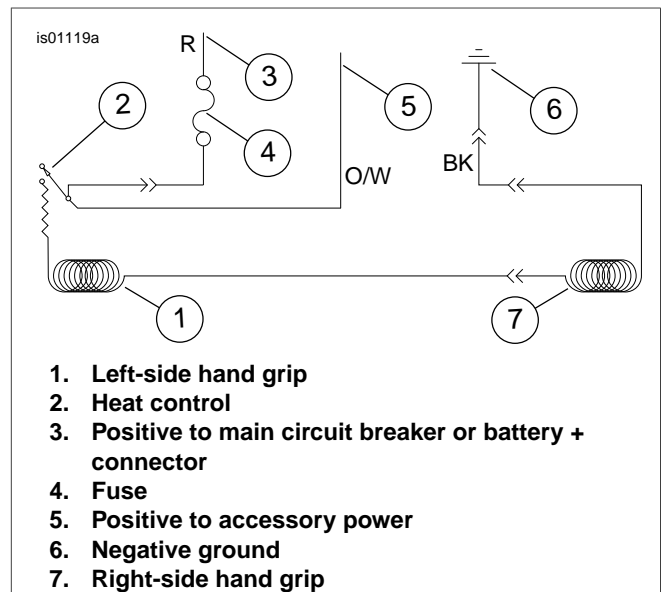
Figure 21. Heated Hand Grip Schematic
