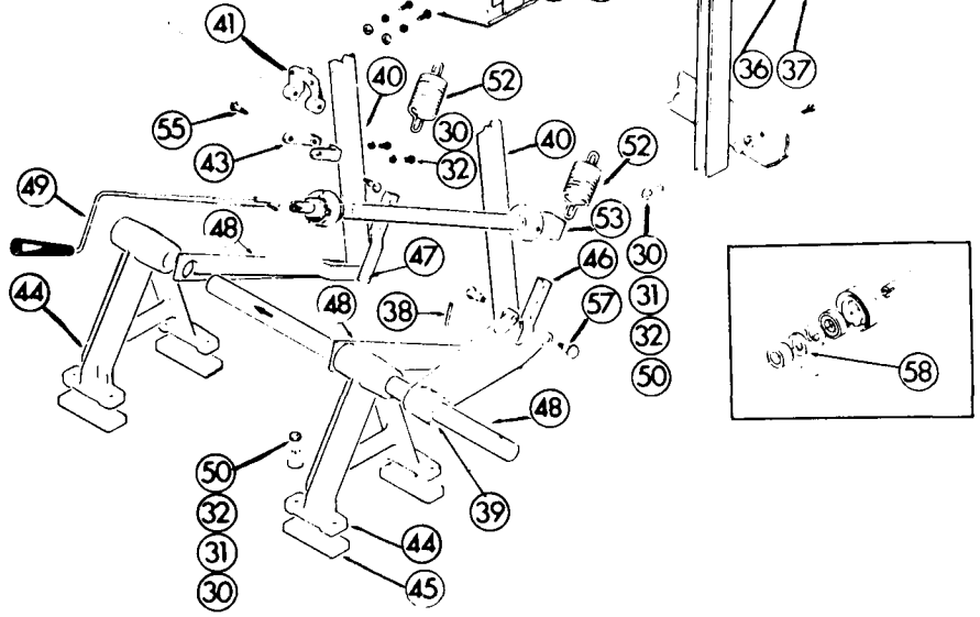
EXPLODED VIEW OF MECHANICAL ASSEMBLY - ELECTRIC - MODEL 1800
