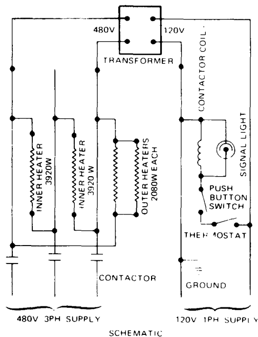
WIRING DIAGRAM - 480 VOLTS A. C. 3-PHASE 60 Hz - TILTING SKILLET - ELECT.
