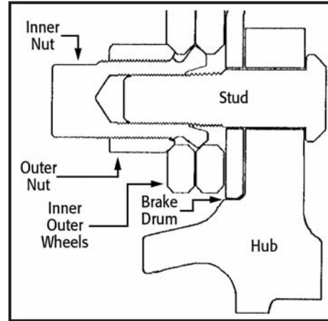
Figure 3 – A ball seat disc wheel mount
